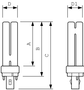
PL-C Xtra 26W/840/2P
