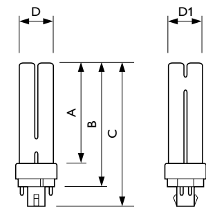
PL-C 18W/830/4P
